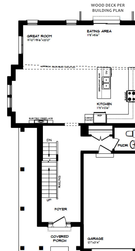
MAIN FLOOR
