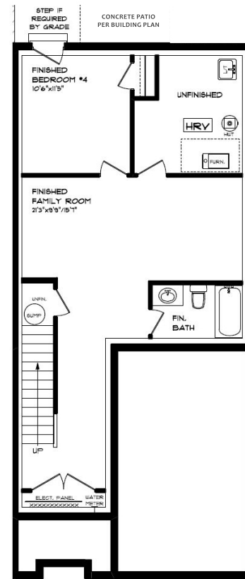
BASEMENT
