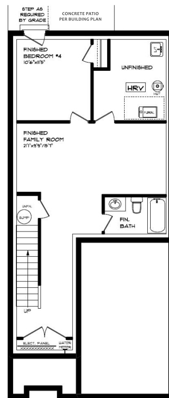
BASEMENT
