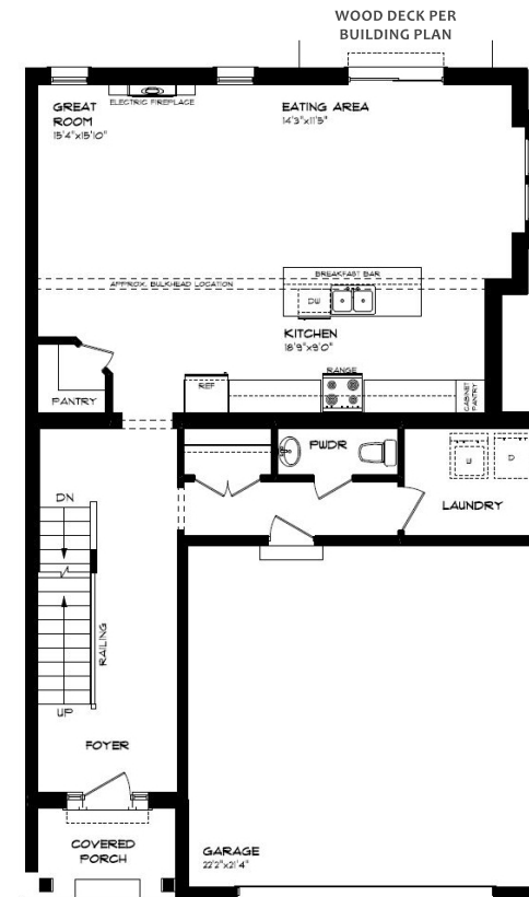
MAIN FLOOR
