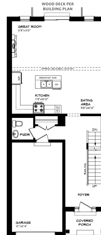
MAIN FLOOR
